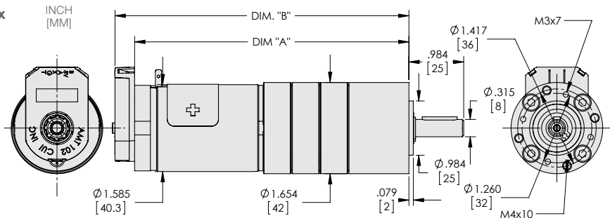
Series 116-8 with Planetary Gearbox & Encoder
